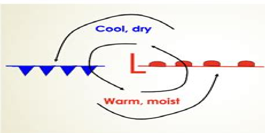
(b) Frontal Wave
