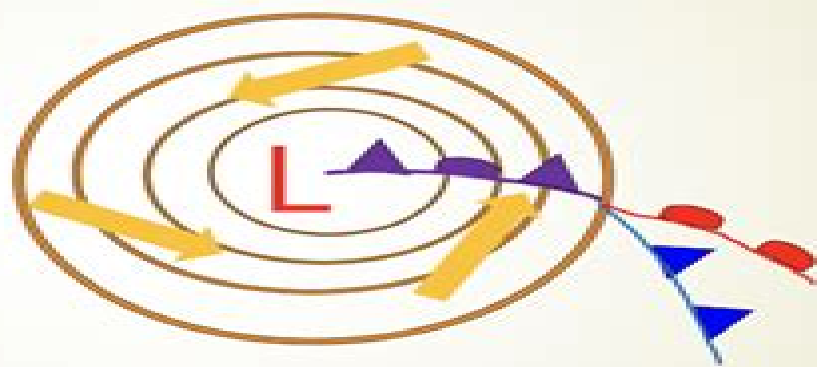
(e) Advanced occlusion
