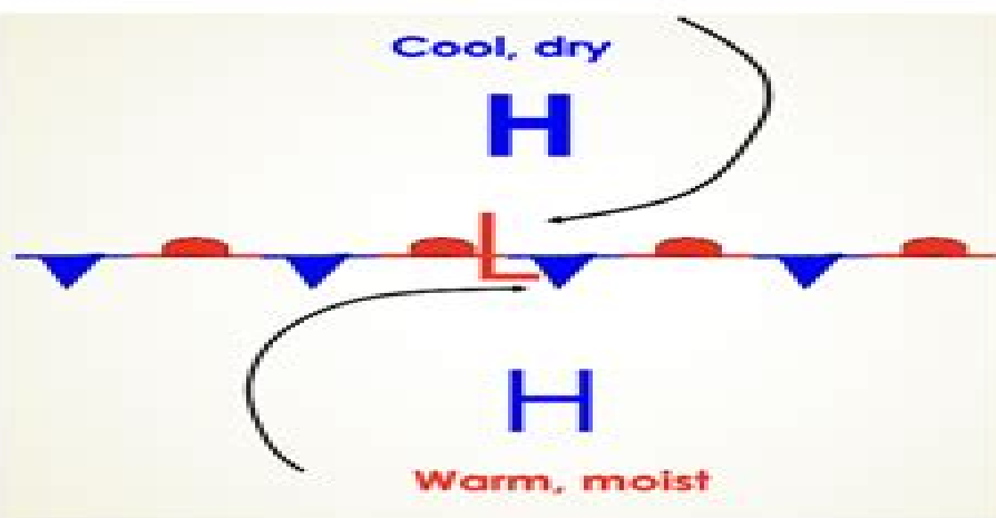
(a) Stationary front
