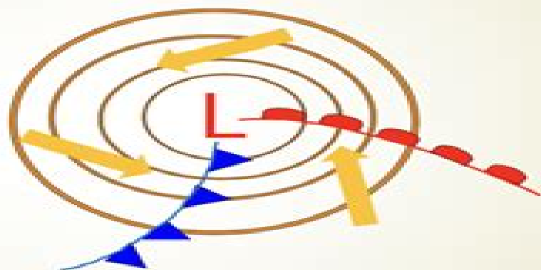
(c) Open Wave
