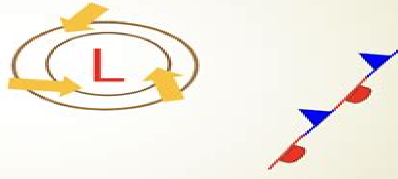
(f) Cut-off cyclone
