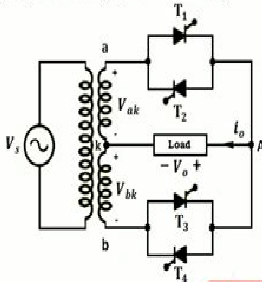
Figure 5 Single phase mid point type rectifier with R
