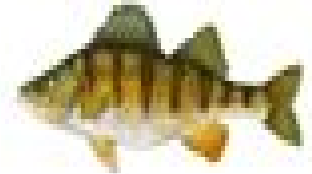
Perch
