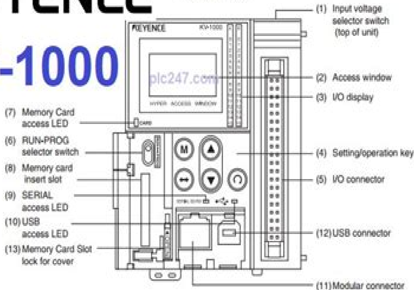
CPU Unit bottom
