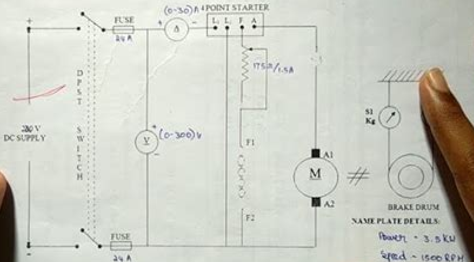
Figure 3-1 - Load Test on DC Compound Motor
