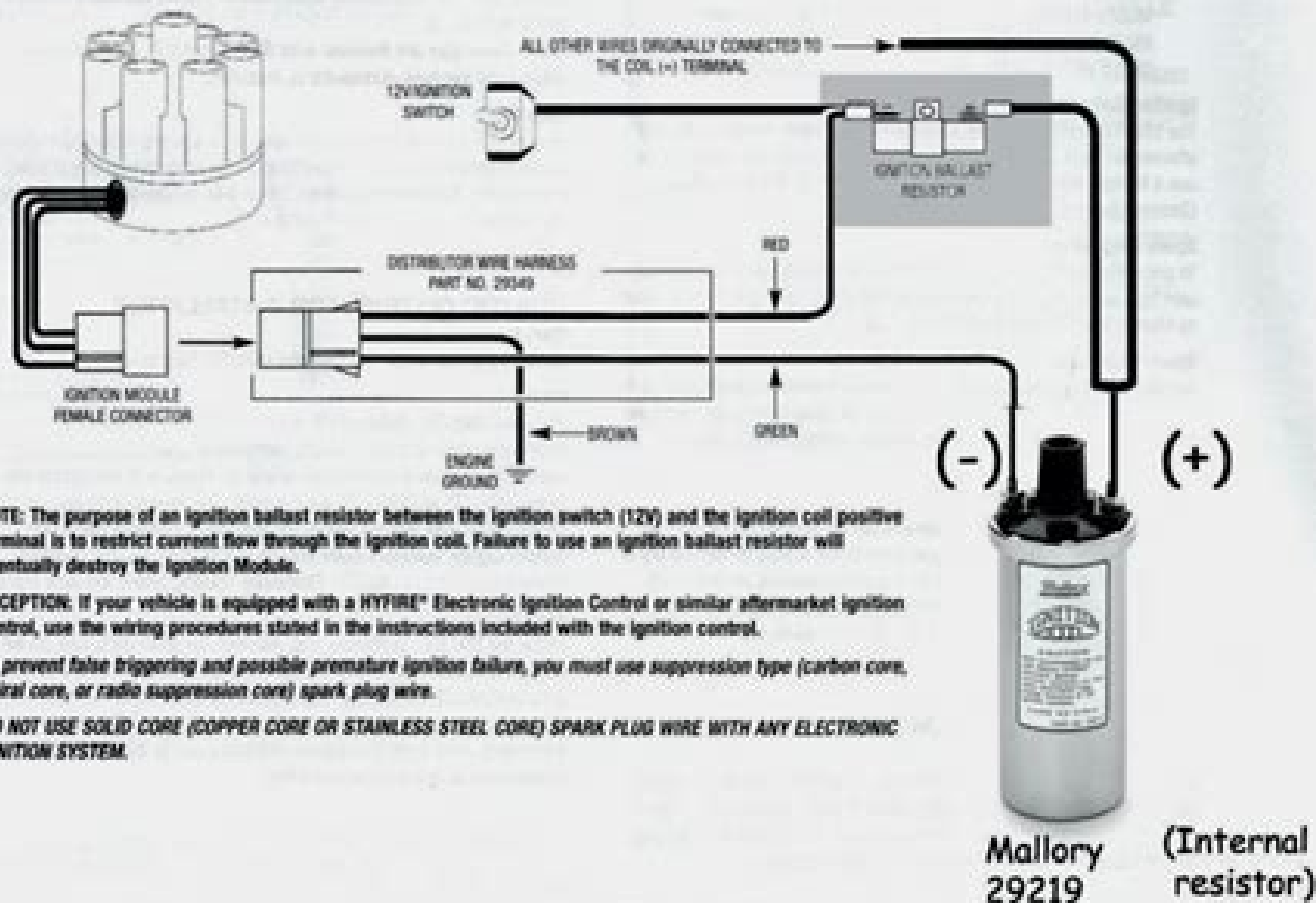
FIGURE 1 UNILITE® WIRING DIAGRAM USING BALLAST RESISTOR
