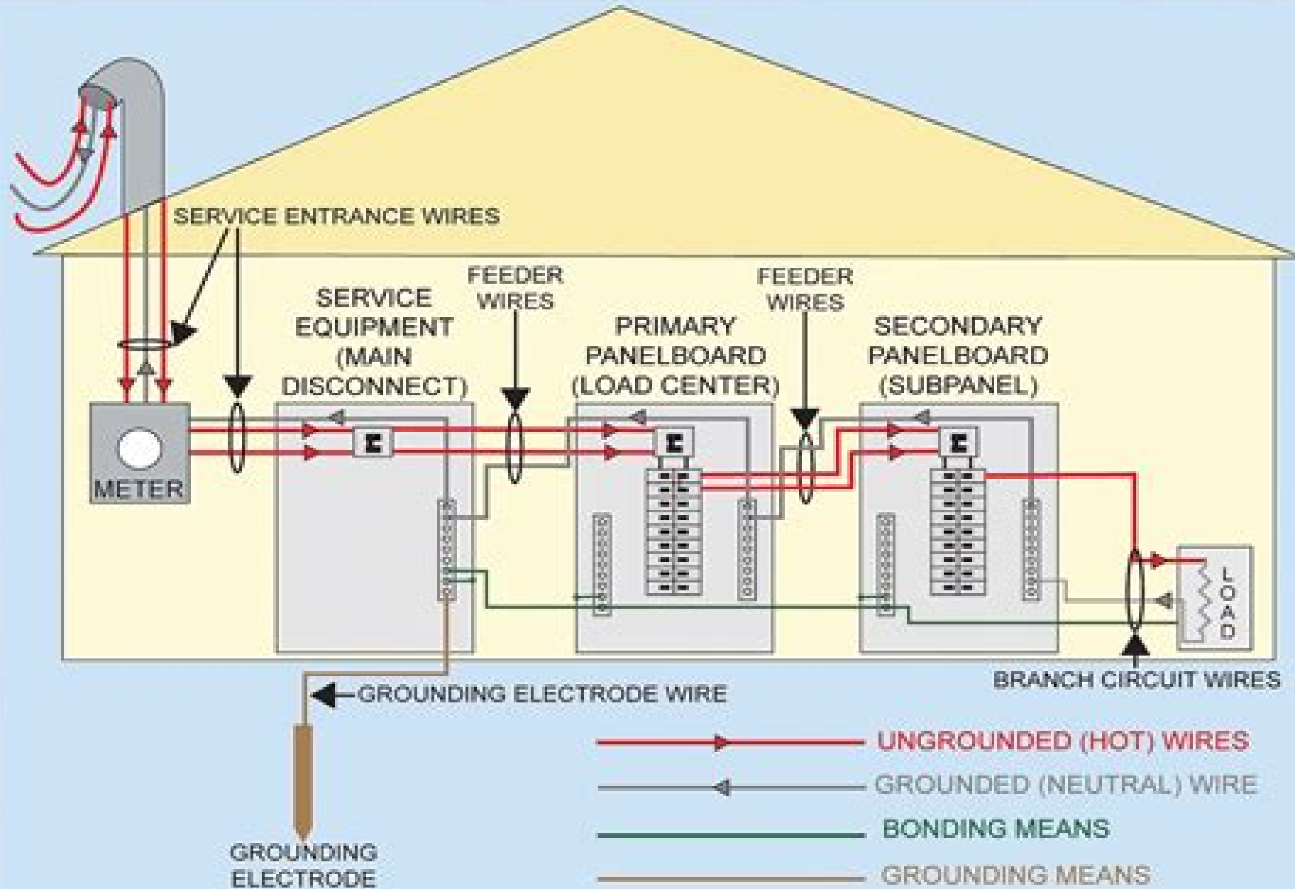
Service Grounding with Separate Service Equipment
