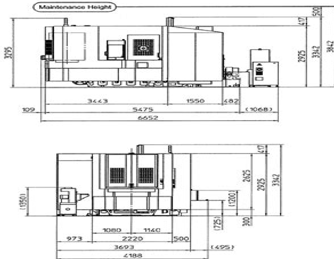
Figure 2.1 Front and Side View of Machine: a81 (Tool Magazine A40 and Left Discharge Lift-Up Conveyor Spec.)
