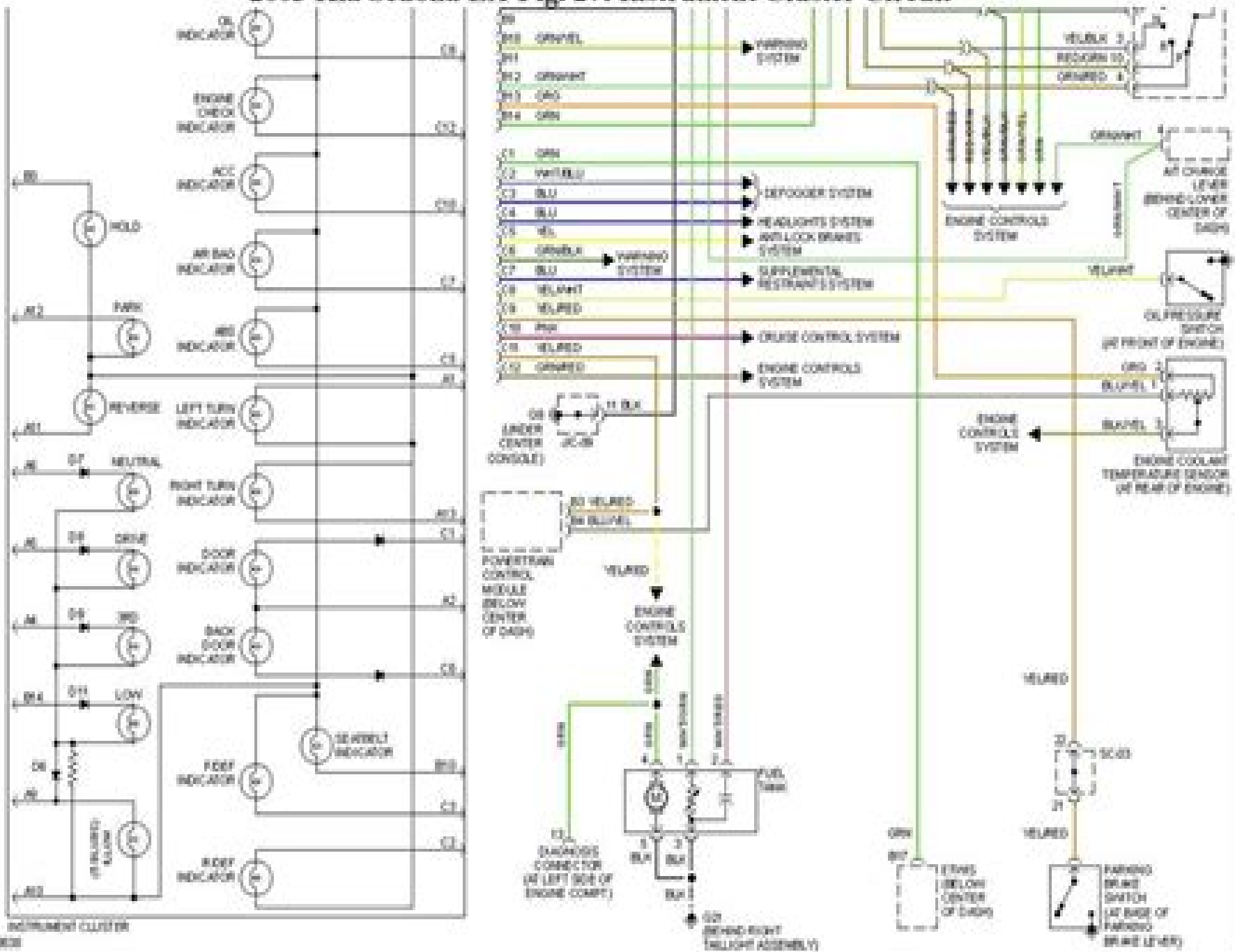
2003 Kia Sedona EX-Fig. 27: Instrument Cluster Circuit
