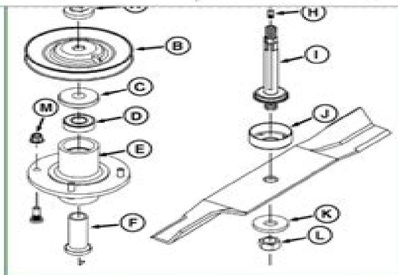
MXT004855-UN: Spindle Starting Model Year 2010 shown.
