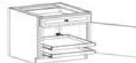
Base Single Door w/Two Full Width Trays (B, 42 1/2") Available sizes: Width: 12, 15, 18, 21, 24 Depth: 24 Height: 34 1/2
