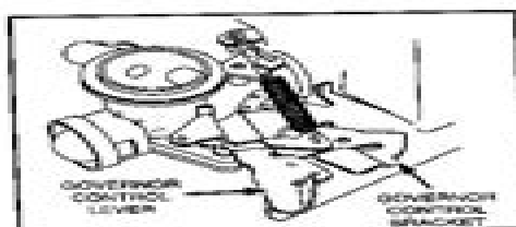
Fig. 55 - Manual Friction
