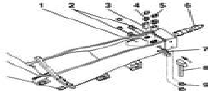
Fig. 1 Removing the working tool
