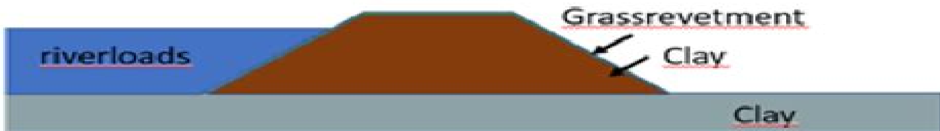
d) Ductile dike with clay
