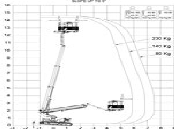
J88B 1450 (21V) LTH WORKING DIAGRAM LATERAL SIDE SLOPE UP TO 15°
