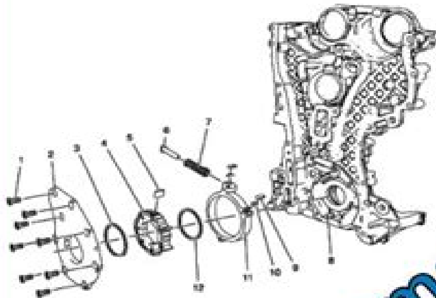
Fig. 3: Engine Front Cover And Oil Pump Assembly. Courtesy of GENERAL MOTORS COMPANY
