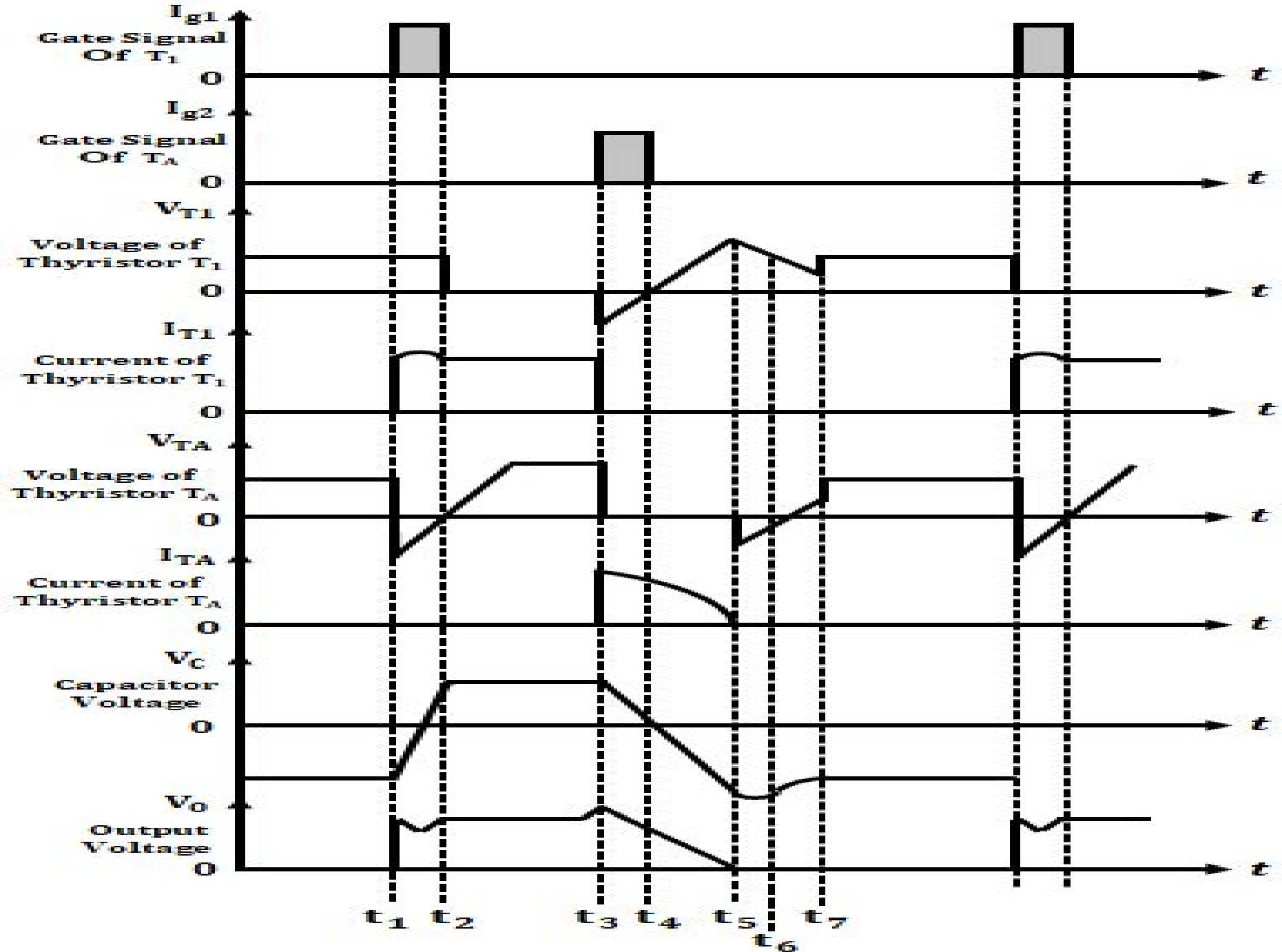
Jones Chopper Voltage and Current Waveforms
