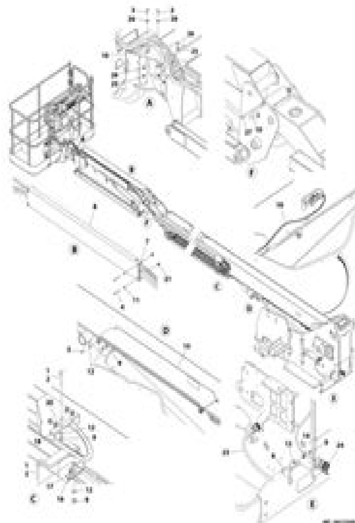
FIGURE 8-33. CABLES AND CLAMPS INSTALLATION - 400LJ (3500W GENERATOR OR NO GENERATOR)
