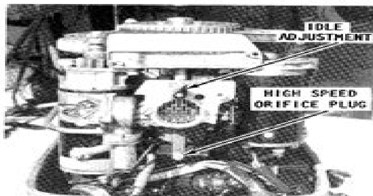
A 40hp powerhead with the idle adjustment screw and the high speed orifice plug identified.
