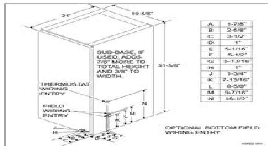
FIGURE 1: Furnace Dimensions
