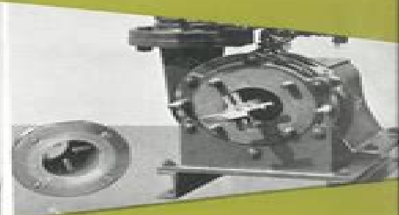
Pump with Suction Inlet removed showing Cutters
