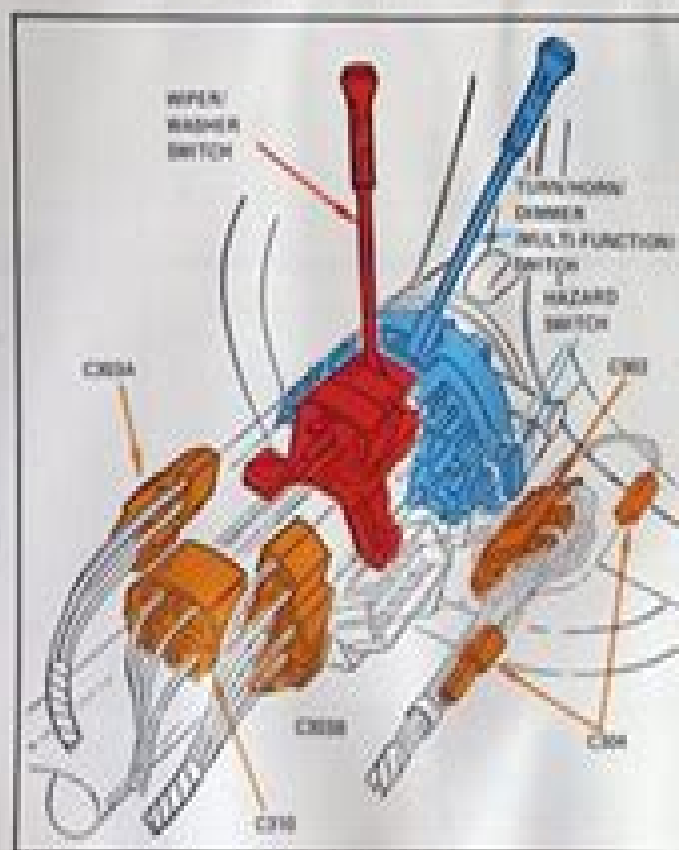
Figure 1 - Steering Column
