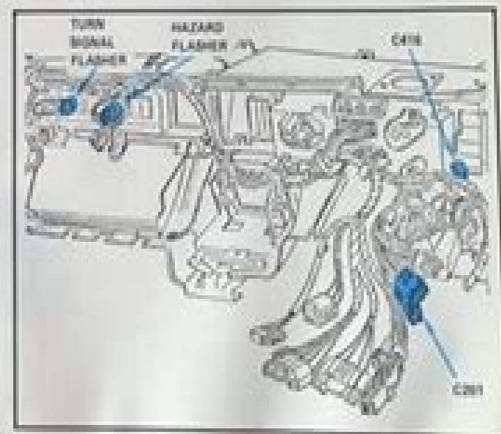
Figure 2 - Back of Instrument Panel
