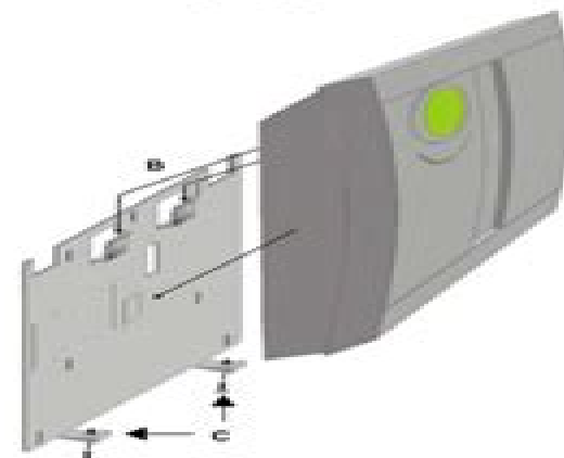
Figure 16: Magellan's Back Plate
