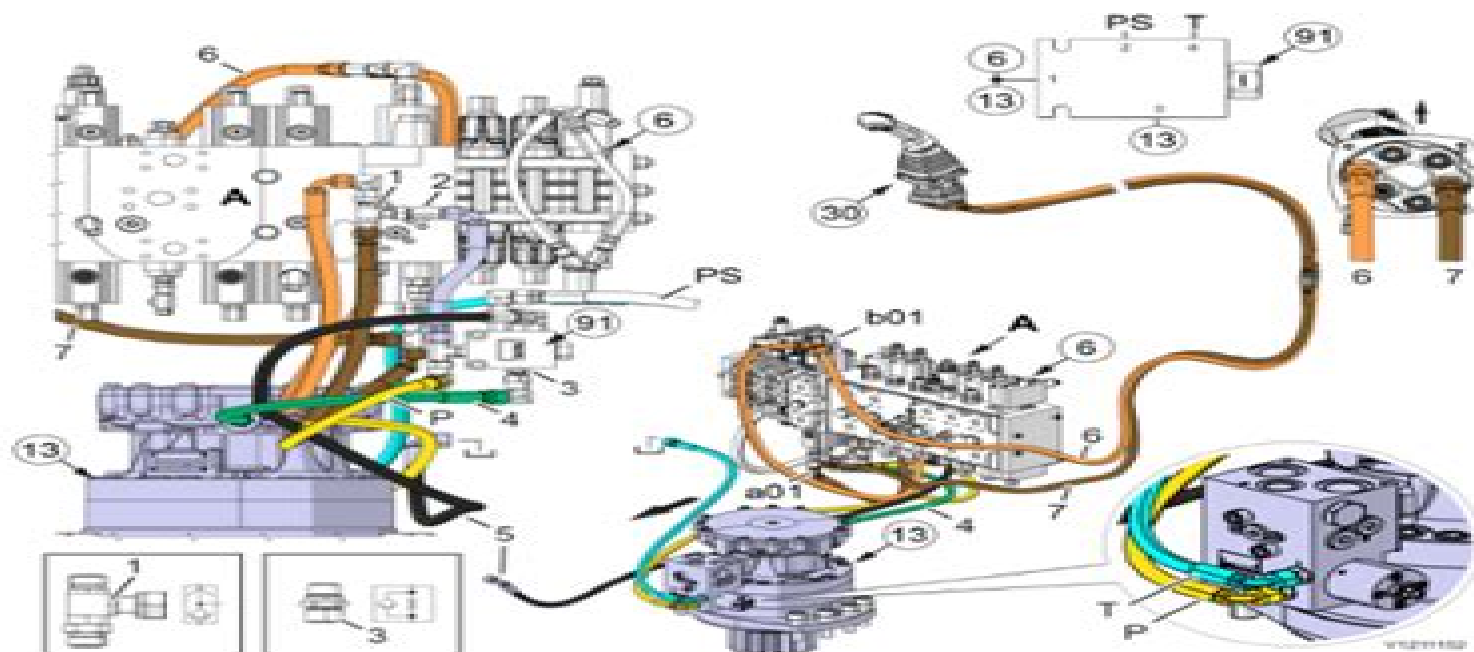
Figure 1006 Swing system main parts
