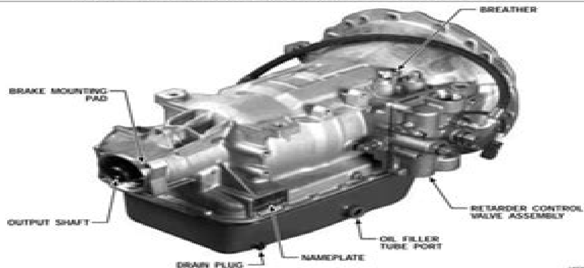
Figure 1-2. AT 545R Automatic Transmission — Right-Rear View
