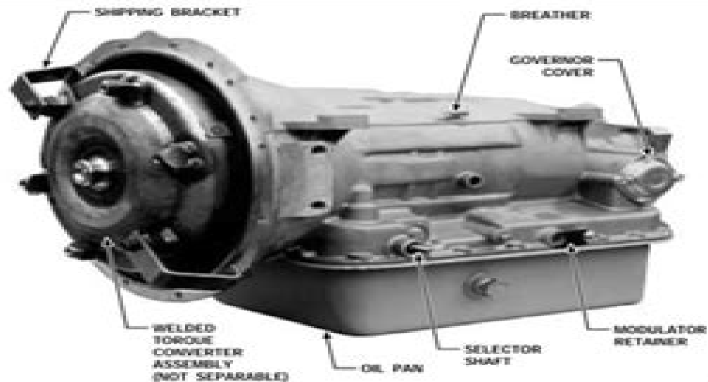
Figure 1-1. AT 1545 Automatic Transmission — Left-Front View
