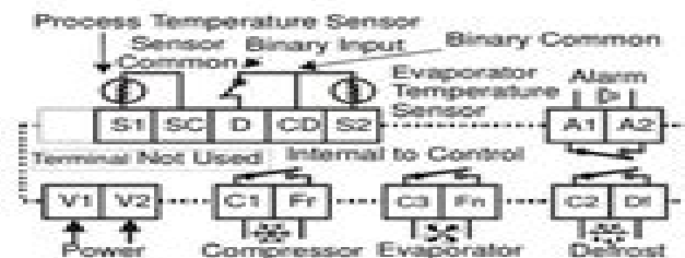
Figure 1: MR4 DIN Rail Mount Control
