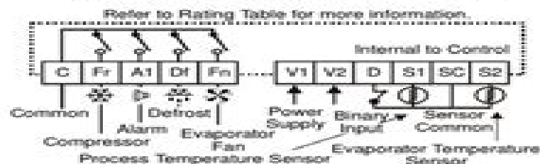
Figure 2: MR4 Panel Mount Control
