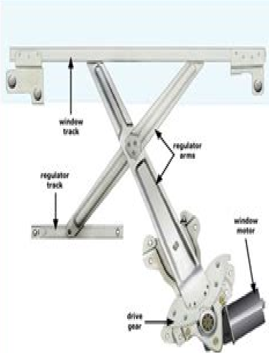
Gear Driven Window Regulator
