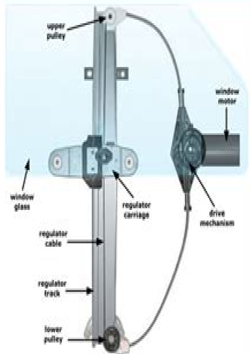
Cable Driven Window Regulator
