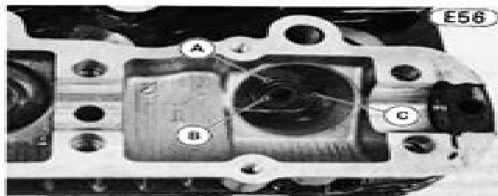
A. Spring Band B. Oil Seal C. Spring Seat
