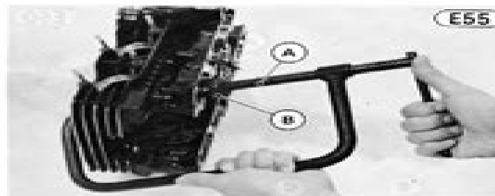
A. Valve Spring Compressor Assembly (57001-241) B. Adapter (57001-243)
