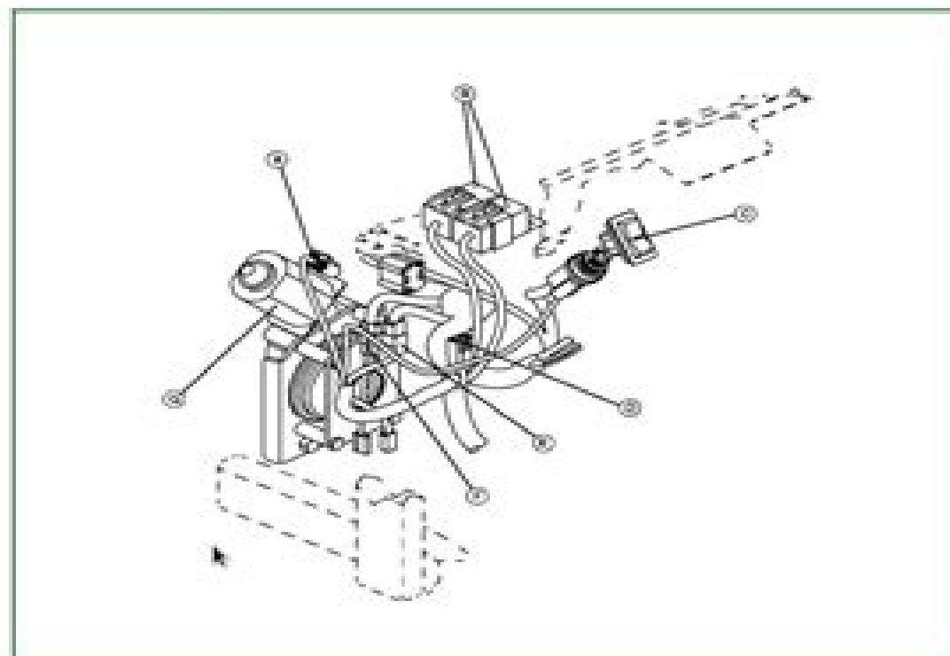
MXAL31909-UN: Front Blade Kit Component Location
