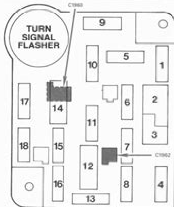
Figure 1 - Fuse Panel
