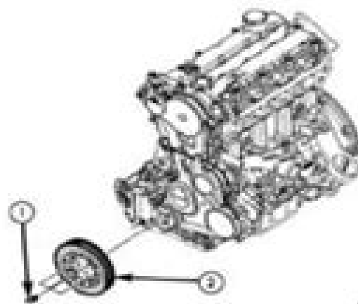
Fig. 12: Crankshaft Damper & Bolts Courtesy of CHRYSLER GROUP, LLC
