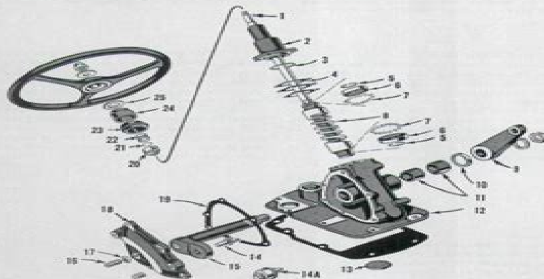
Fig. MF237—Exploded view of the cam and lever type steering gear unit used on models F40, MH50 and MF50. Camshaft bearings and lever backlash are adjustable.
