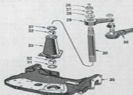
Fig. MF239—Exploded view of the upper pedestal and components used on models F40, MH50 and MF50 with manual steering.
