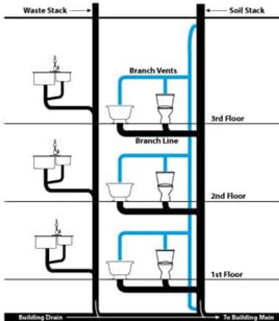
Multi-story Drainage and Venting
