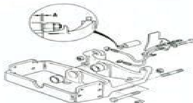
Fig. 12—Measure gap (A) between the top spacer tube on right side and front support of 340-360 models.
