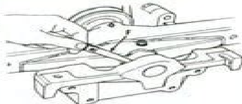
Fig. 10—End play of front axle should be measured with a feeler gauge as shown for 340-360 models with two-wheel drive.
