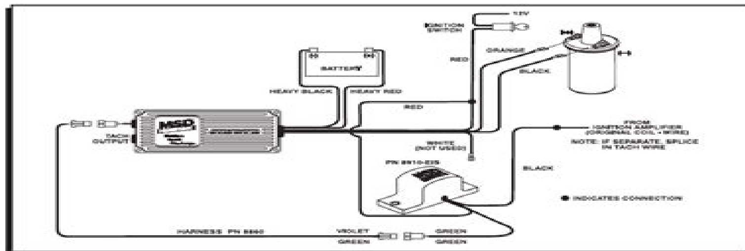
Figure 1 Wiring the Tach Adapter.
