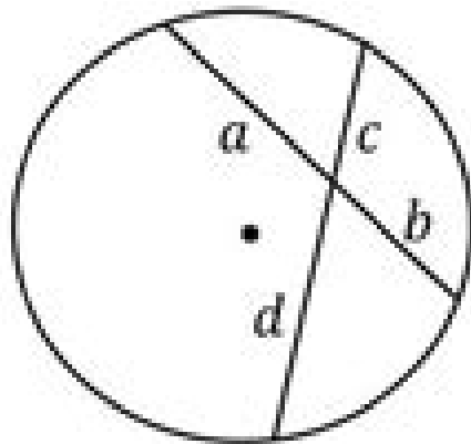
2 Chords
