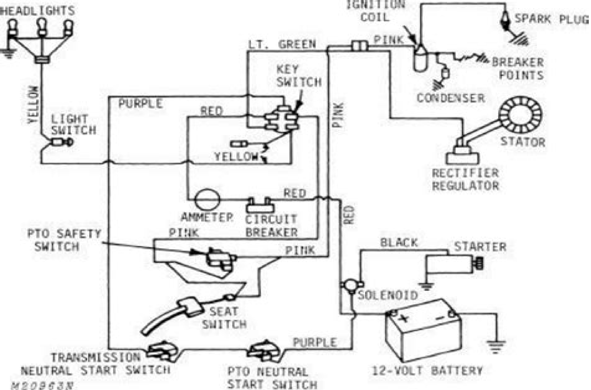
Fig. 3-Wiring Diagram For 210, 212, 214 and 216 Tractors (Serial No. 70,001-190,000)
