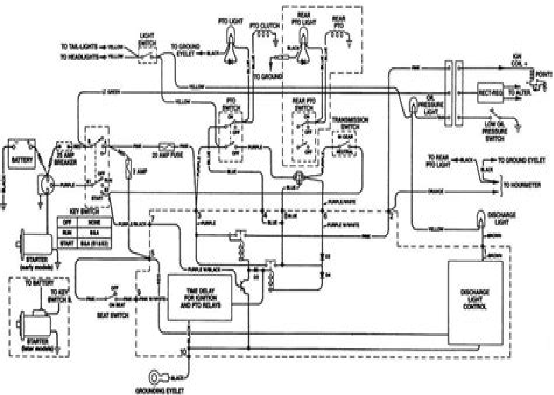
46-22-Wiring diagram for Model 316.
