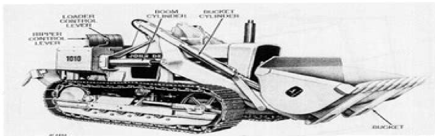
John Deere 1010 Crawler Loader and 35 Hydraulic Ripper (Manufactured 1960-1964)
