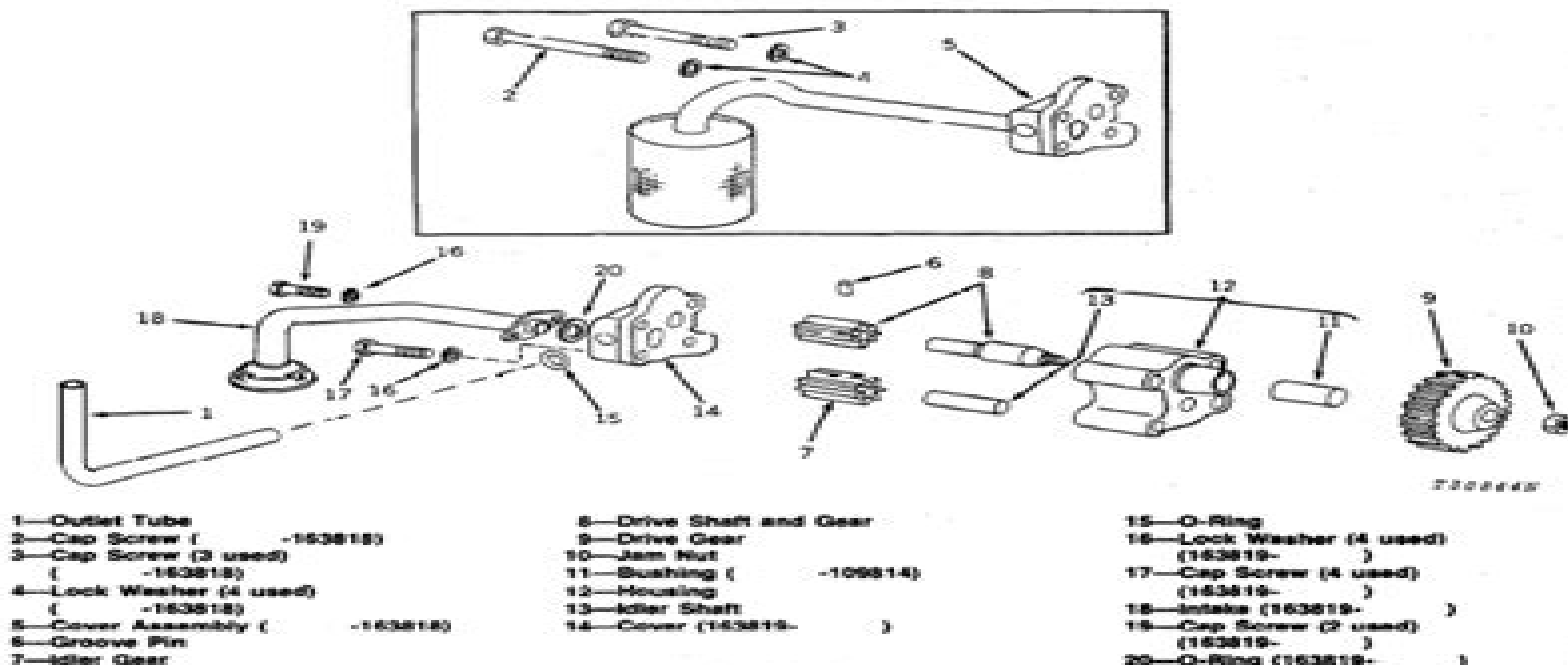
Fig. 3—Oil Pump
