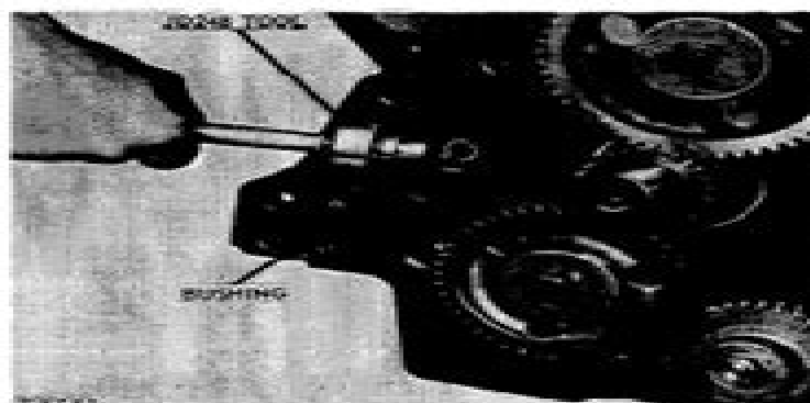
Fig. 4—Installing Pressure Regulating Valve Bushing
