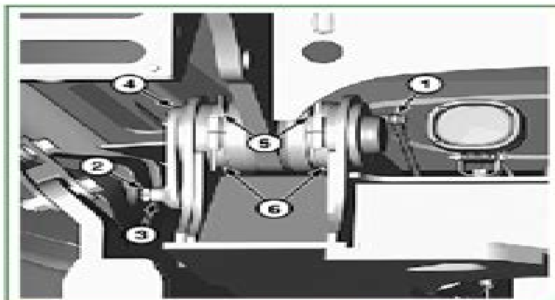
TX1233425A-UN: Dump Body Pivot Pin (left side shown)
