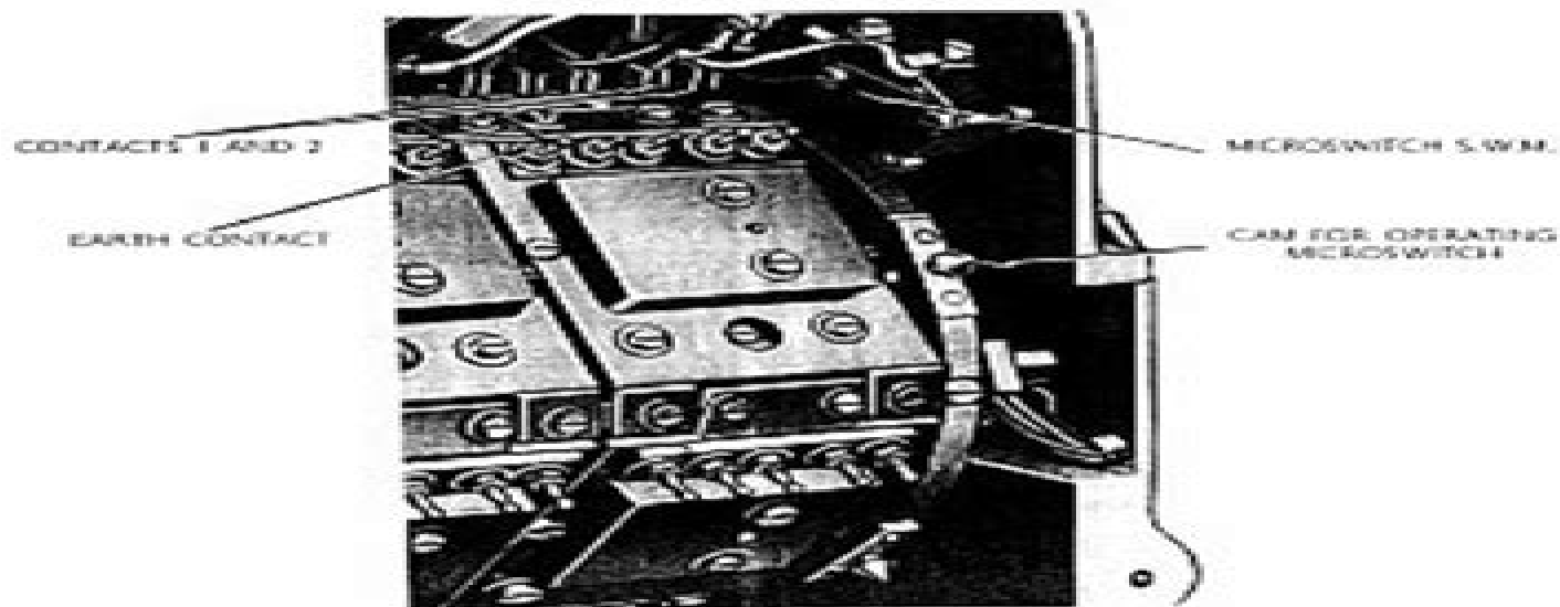
(A) AERIAL TURRET SECTION
