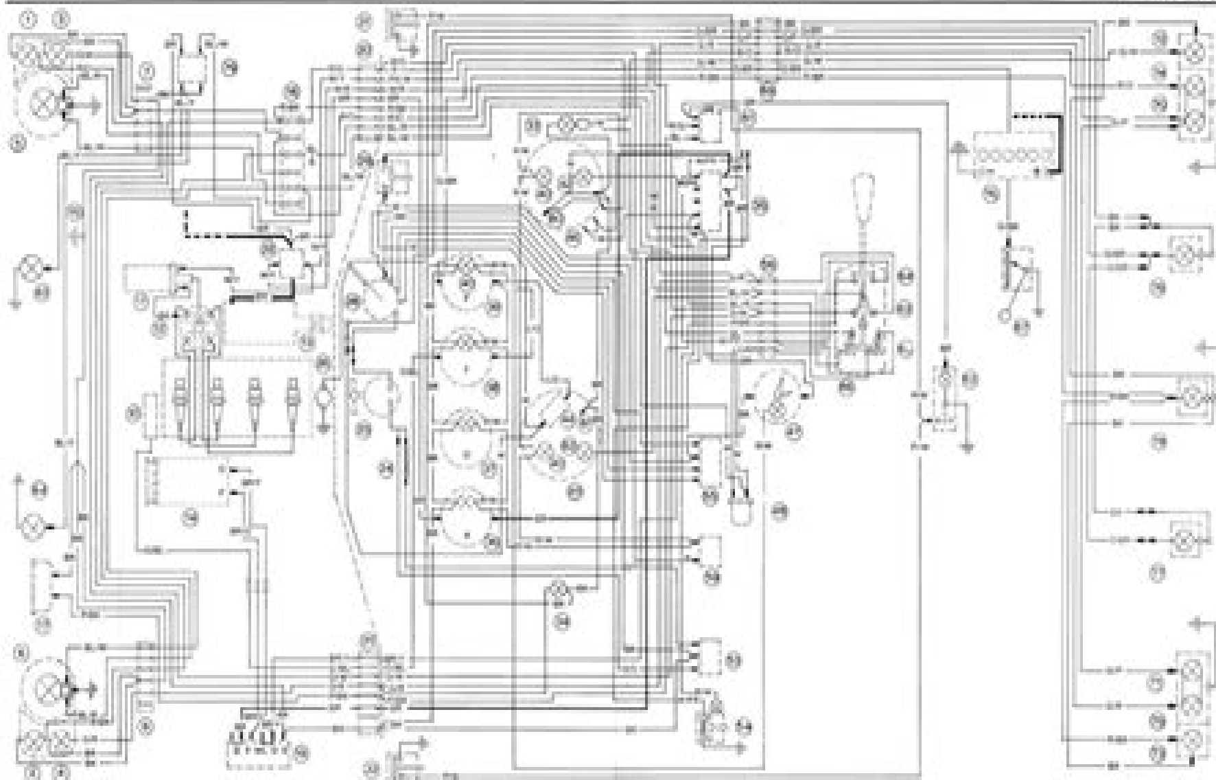
WIRING DIAGRAM - R.H.D. CAR
