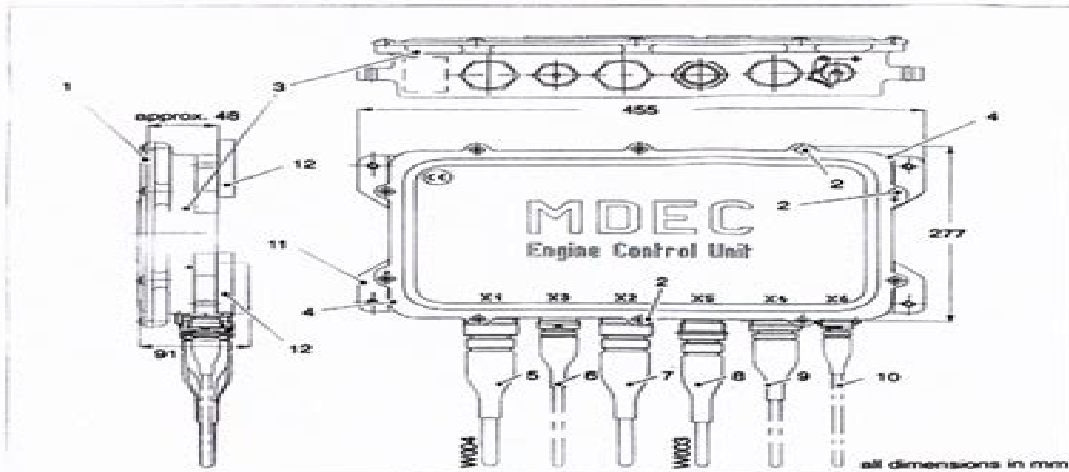
Fig. 67 : Mechanical structure
