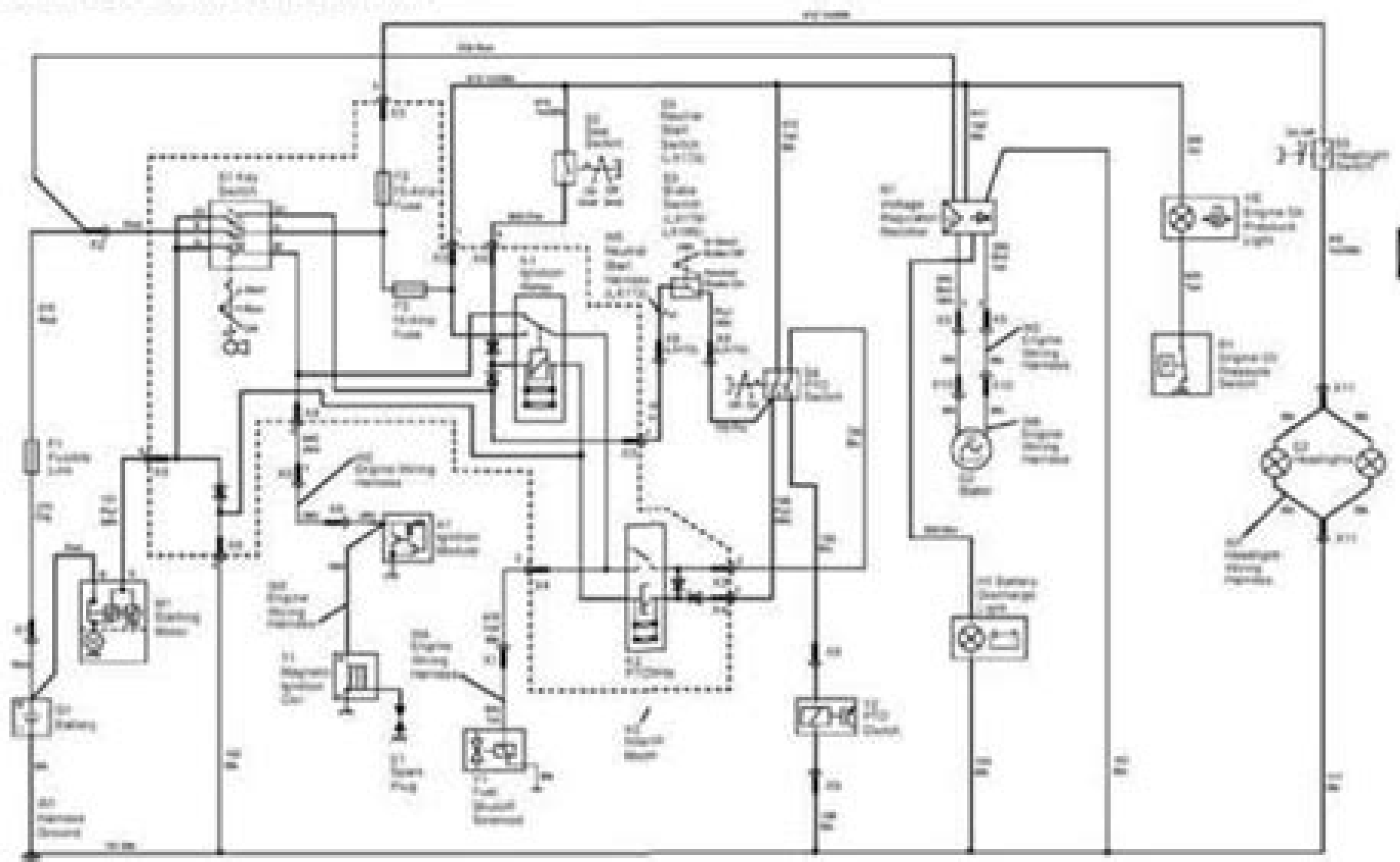
ELECTRICAL SCHEMATIC—LX172/LX176/LX190
