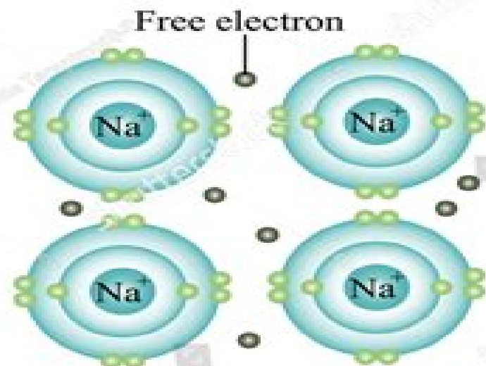
Metallic Bonding
