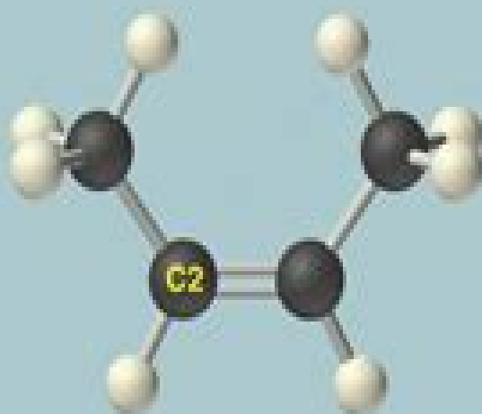
cis -2-Butene, C_4H_8
