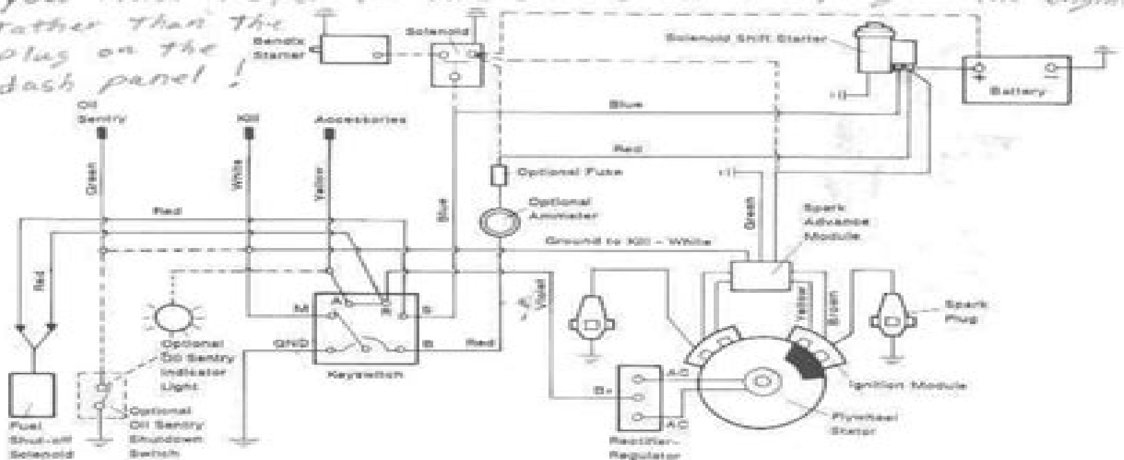
Figure 8-8. Wiring Diagram - 15 amp Regulated Battery Charging System.
