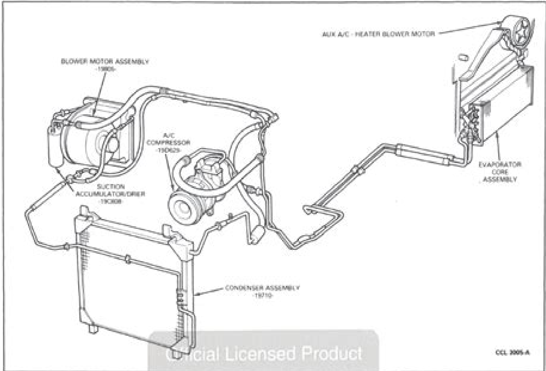
FIG. 2 Typical Auxiliary A/C-Heater System
