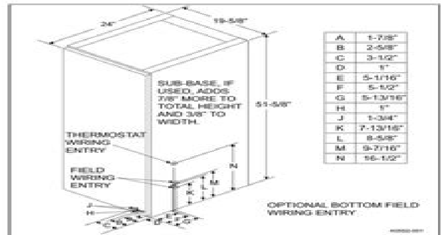
FIGURE 1: Furnace Dimensions
